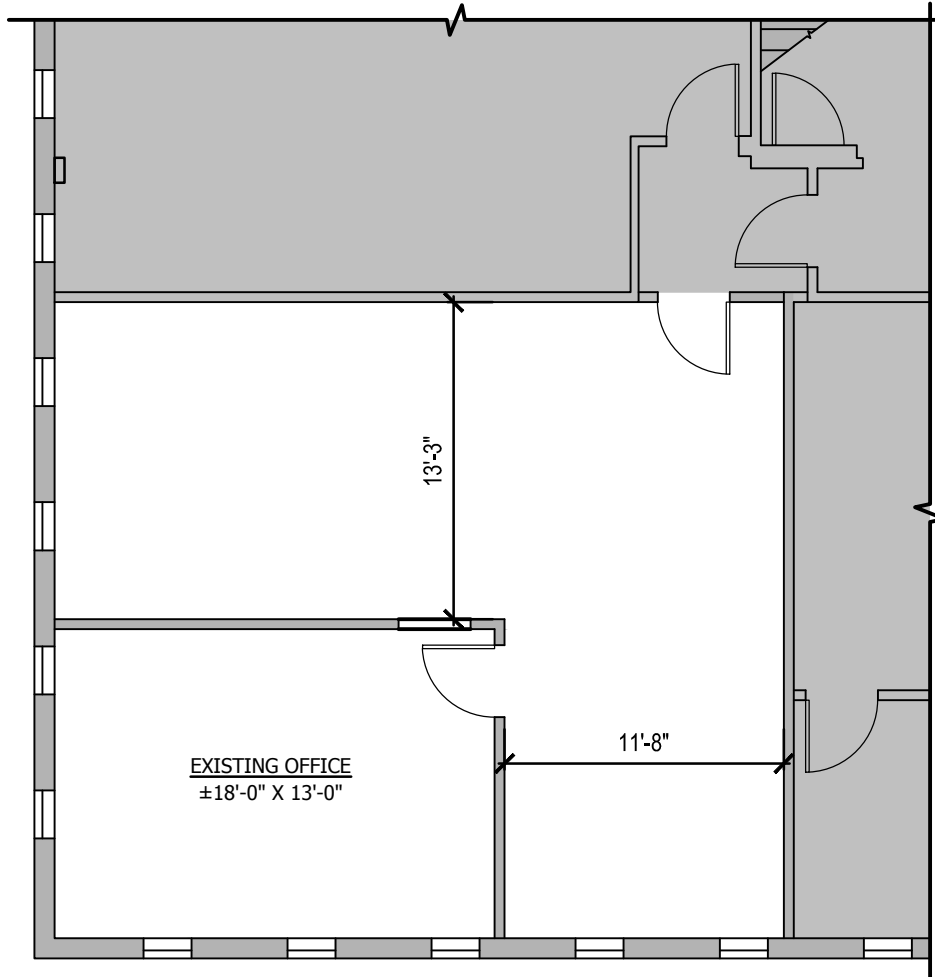
1 SUITE 112 - MARKETING PLAN - 971 RSF SCALE: 1/8" = 1'-0"
