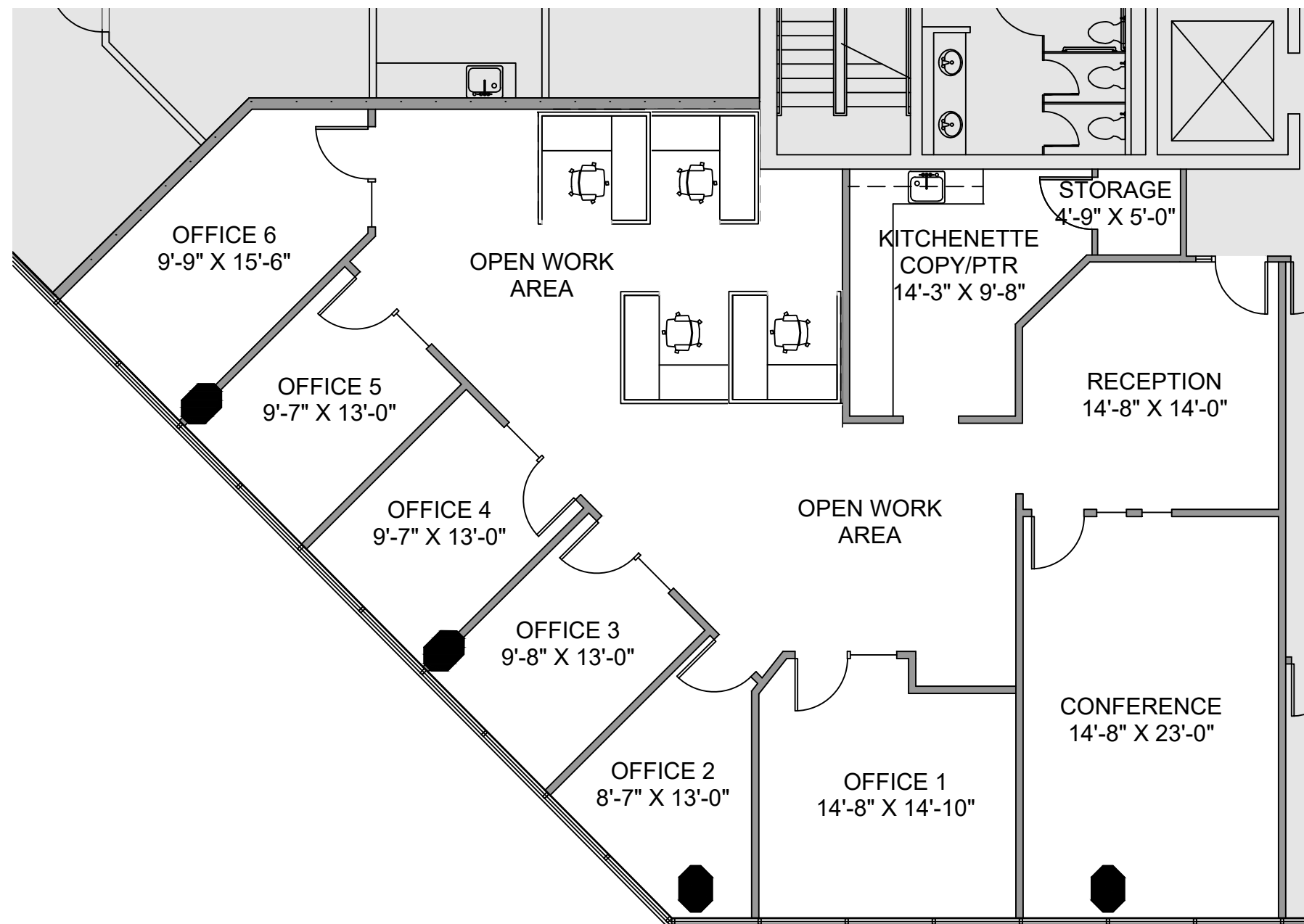
1 SUITE 208 MARKETING PLAN - 2,845 RSF Scale: 1/8" = 1'-0"
